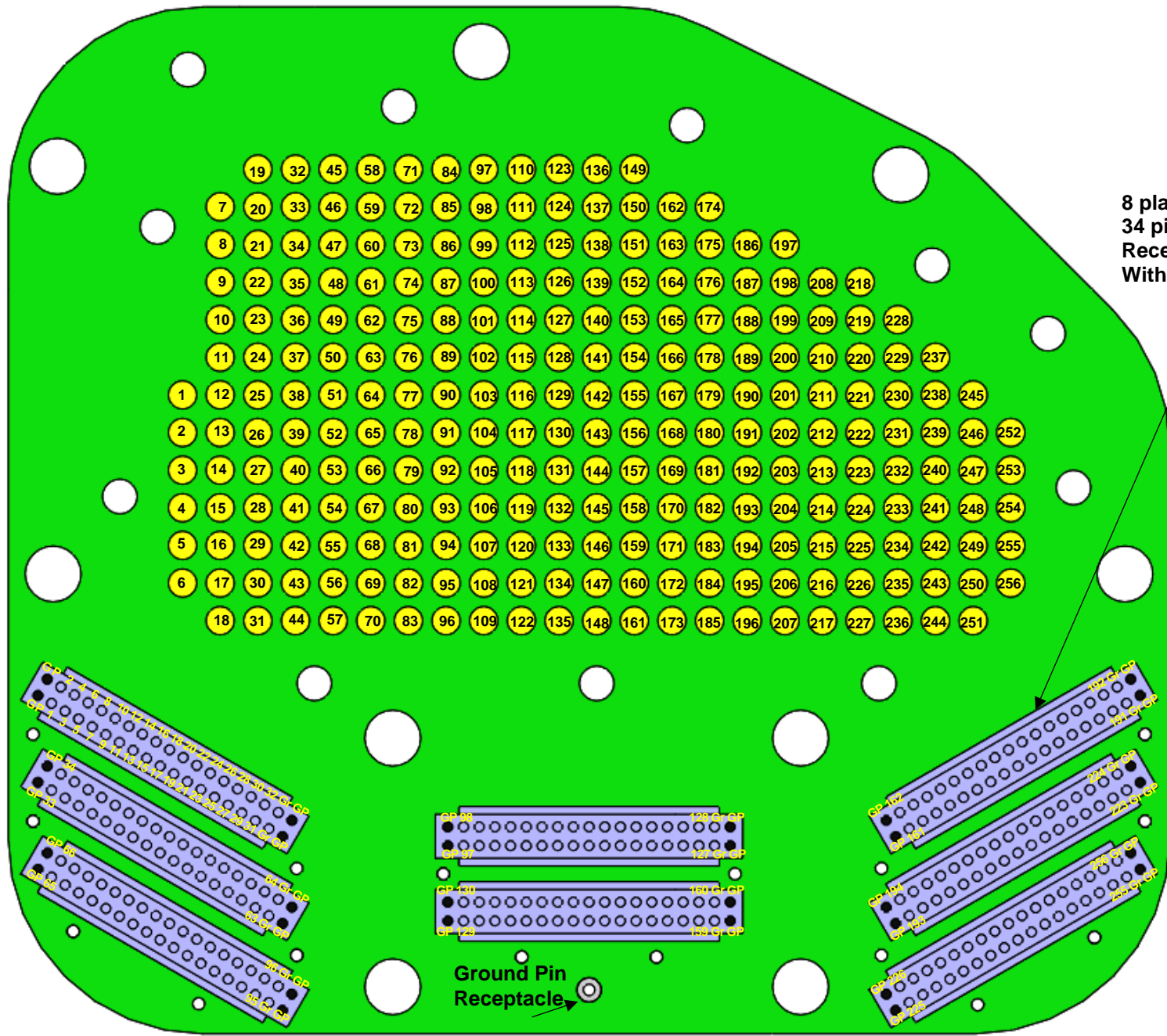
Gray Matter Research – LS256 PCB Schematic
