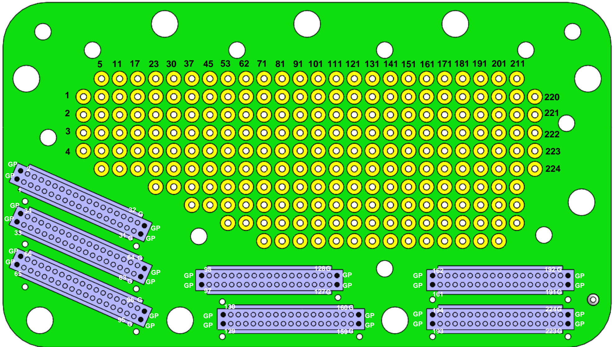
224 channels, seven 32 channel connectors. Each connector has four Guide Pins (GP) and two Ground (G) channels.
