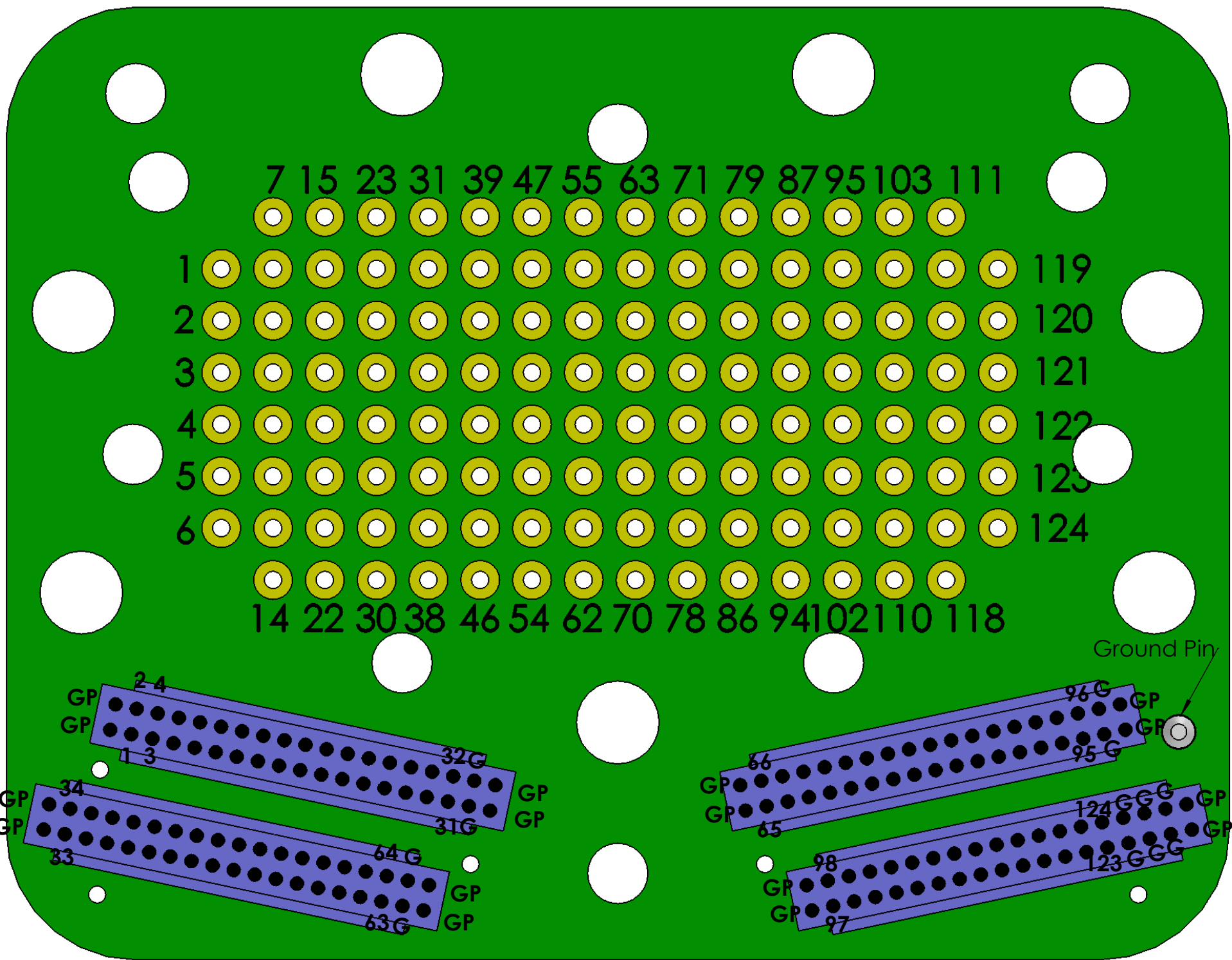
124 channels, Four 32 channel connectors. Each connector has four GuidePins (GP) and two Ground (G) channels.
