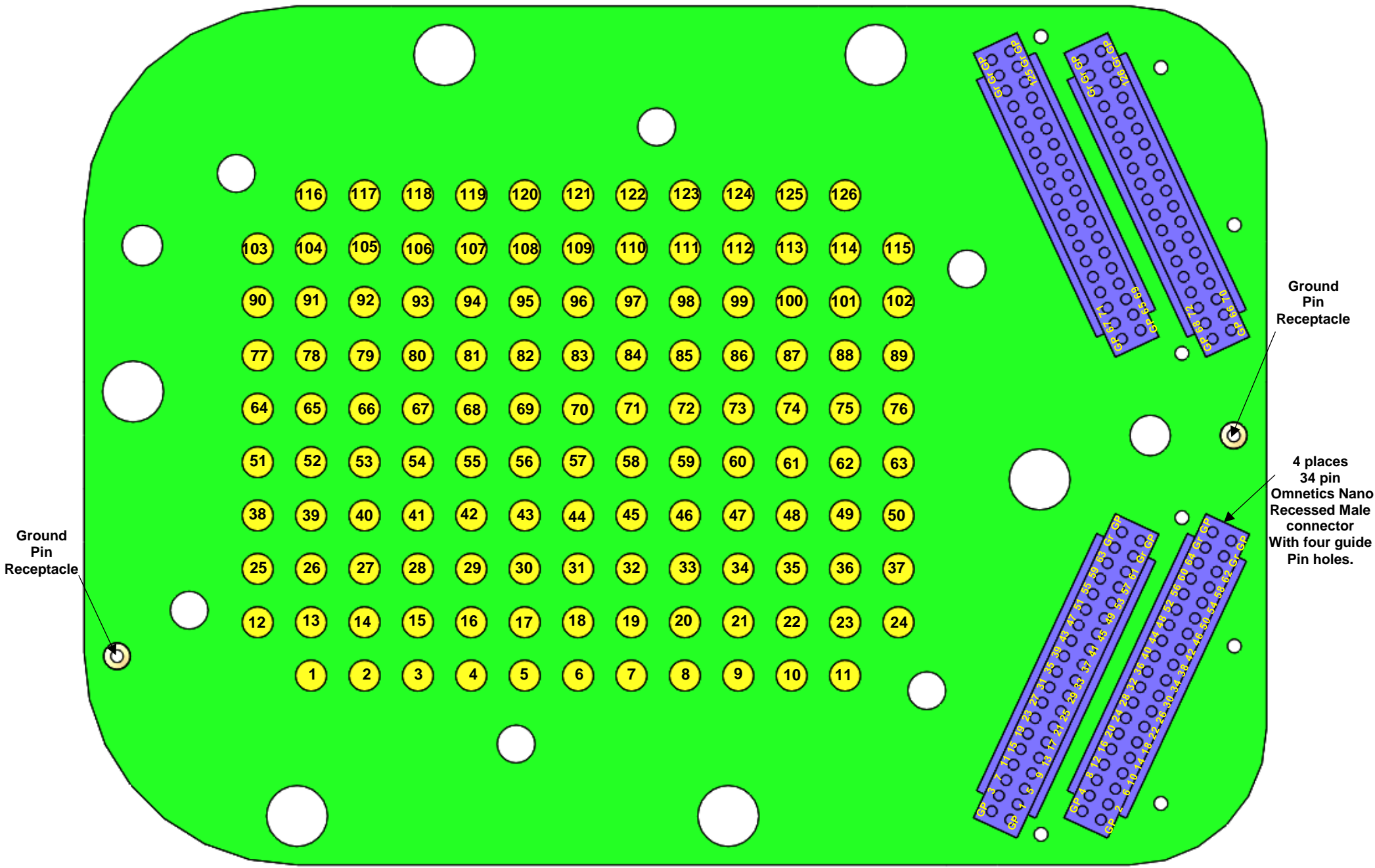
Gray Matter Research – LS126 PCB Schematic
